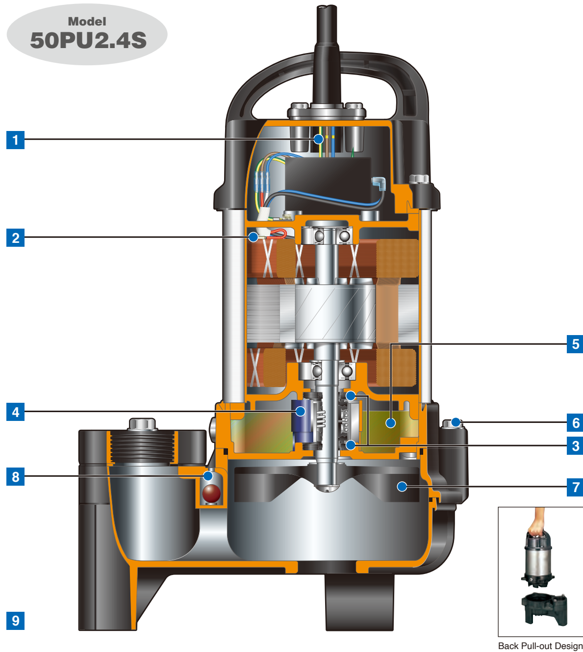
Back Pull-out Design
